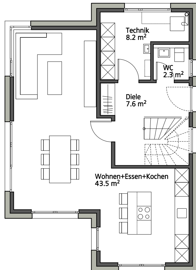
Erdgeschoss Variante A
